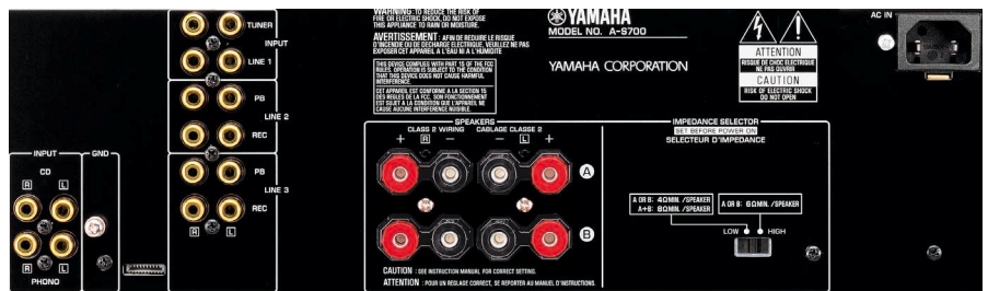
Rear panel is depending on areas. Banana-plug compatible speaker terminals are not available in some areas.
